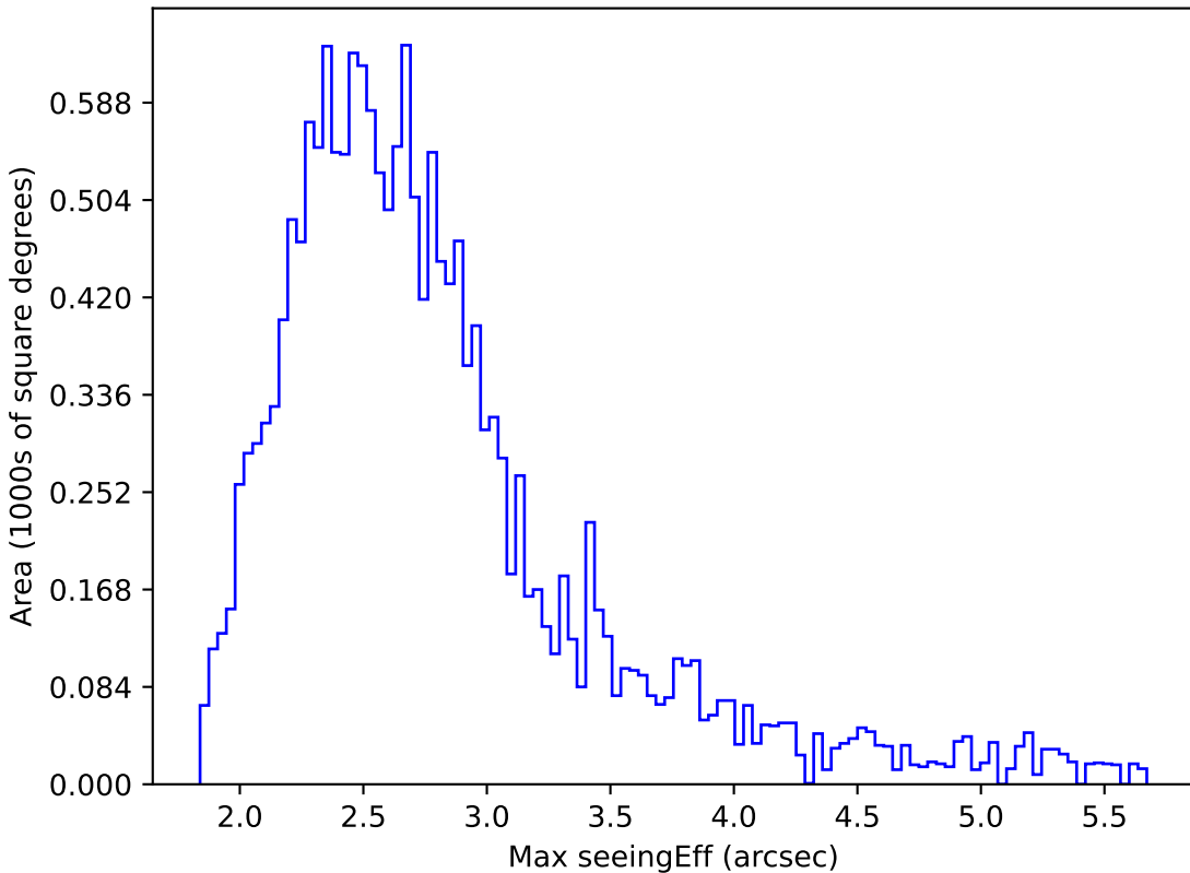
weather_cloudso18v3.4_10yrs WFD z band: Max seeingEff
