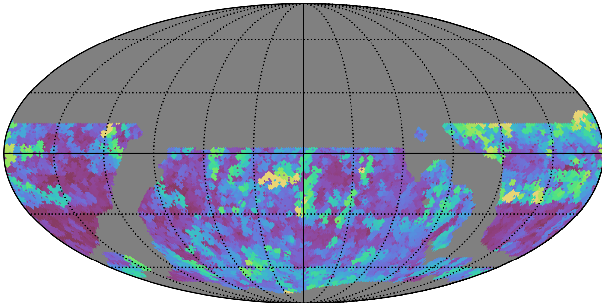
weather_cloudso18v3.4_10yrs WFD r band: Max seeingEff
