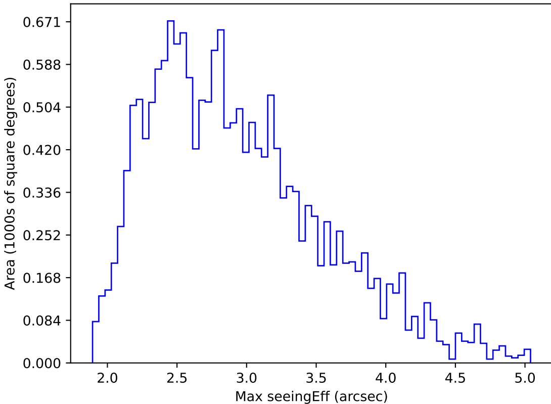
weather_cloudso18v3.4_10yrs WFD r band: Max seeingEff
