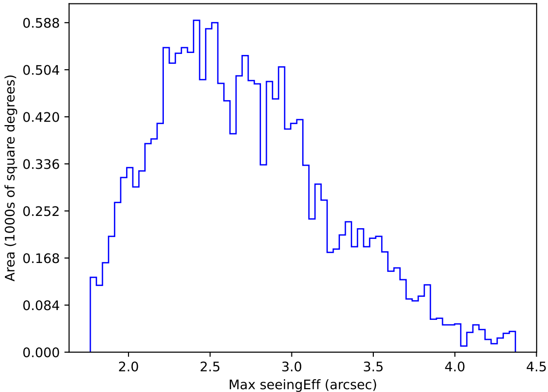
weather_cloudso18v3.4_10yrs WFD g band: Max seeingEff
