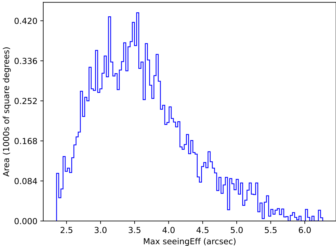
weather_cloudso18v3.4_10yrs WFD all bands: Max seeingEff
