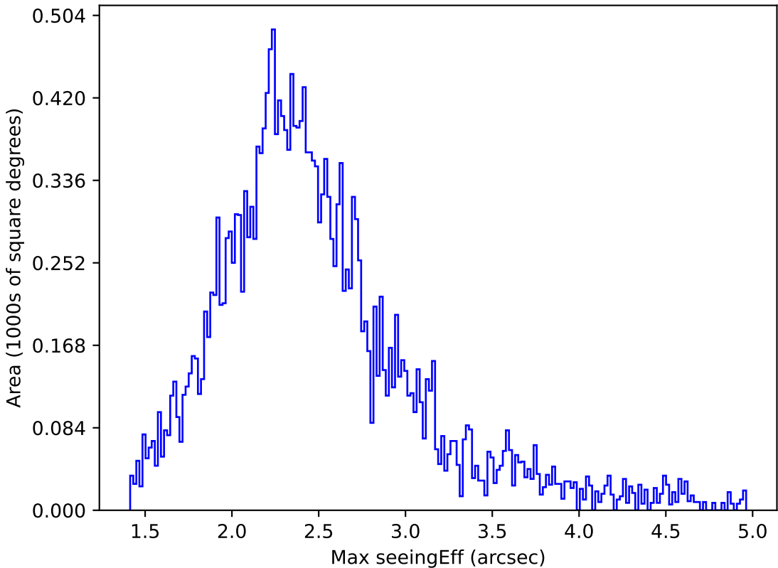
weather_cloudso18v3.4_10yrs All sky y band: Max seeingEff
