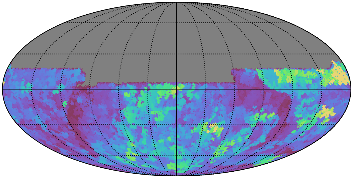
weather_cloudso18v3.4_10yrs All sky u band: Max seeingEff
