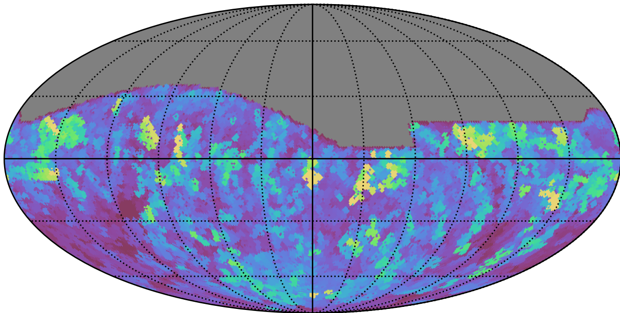
weather_cloudso18v3.4_10yrs All sky i band: Max seeingEff
