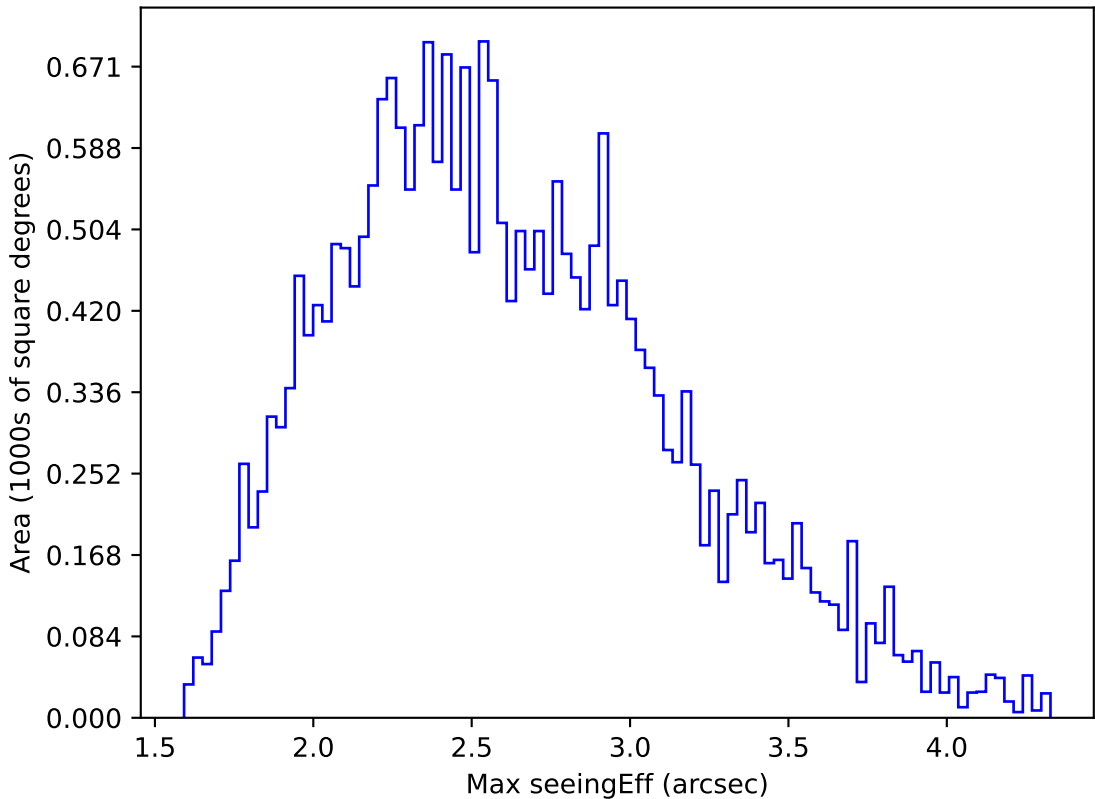
weather_cloudso18v3.4_10yrs All sky g band: Max seeingEff
