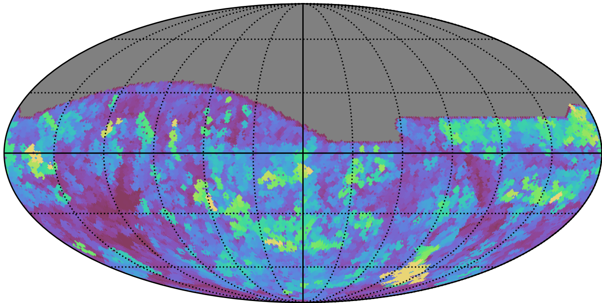
weather_cloudso18v3.4_10yrs All sky all bands: Max seeingEff
