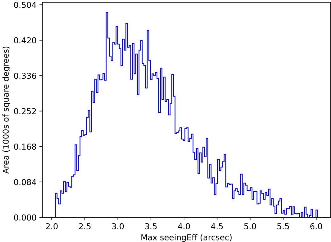
weather_cloudso18v3.4_10yrs All sky all bands: Max seeingEff
