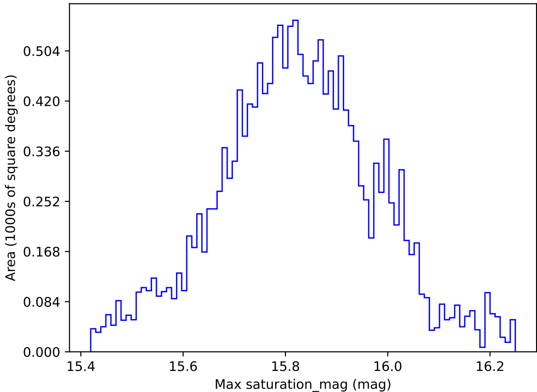
weather_cloudso18v3.4_10yrs WFD all bands: Max saturation_mag
