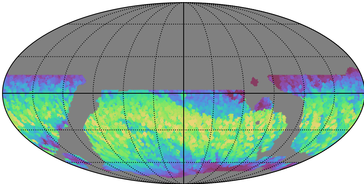
weather_cloudso18v3.4_10yrs WFD all bands: Max normairmass
