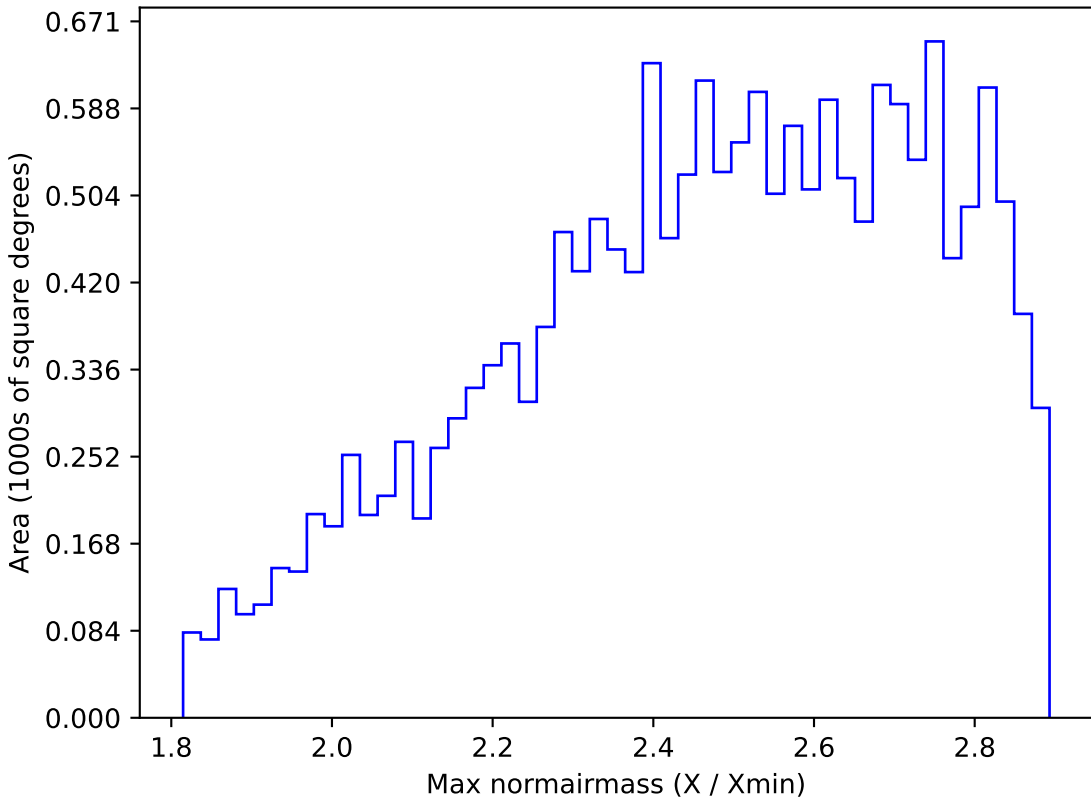
weather_cloudso18v3.4_10yrs WFD all bands: Max normairmass
