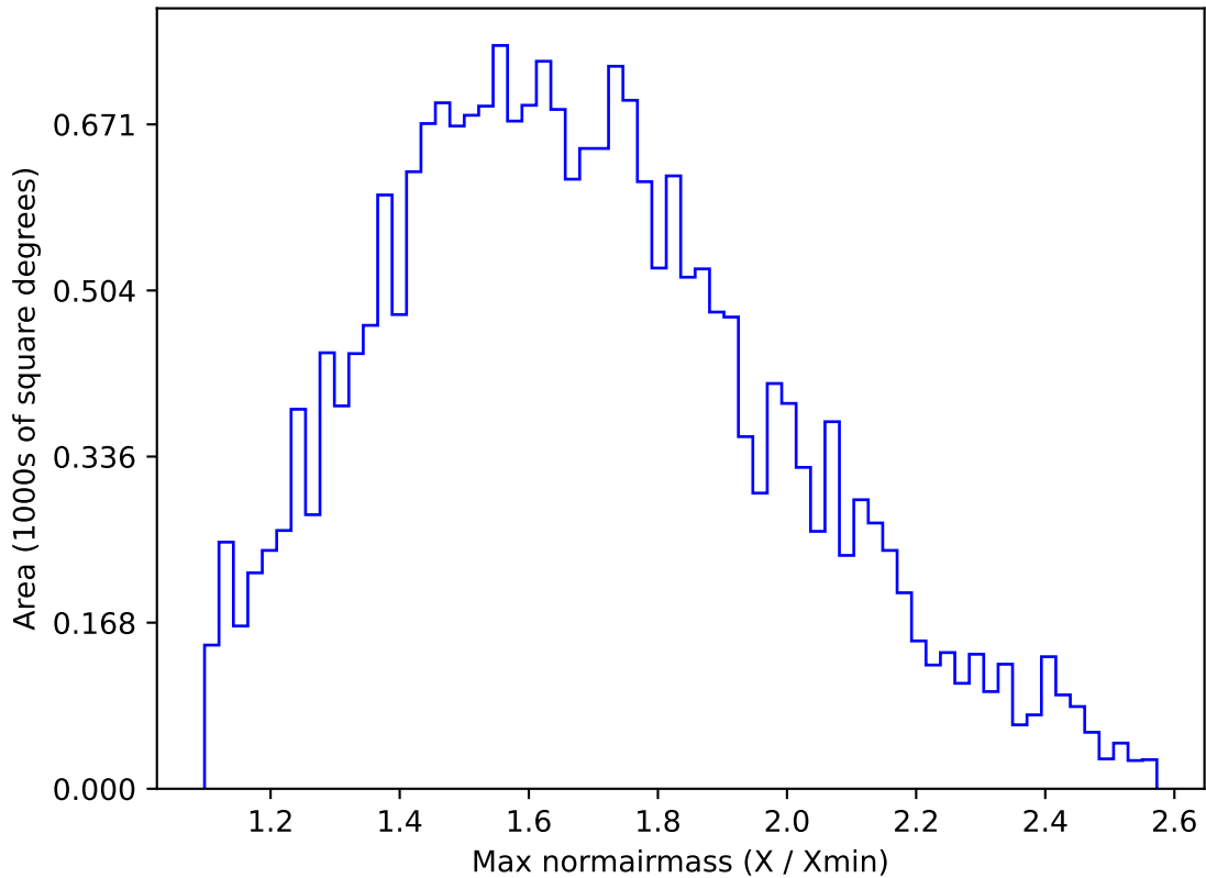
weather_cloudso18v3.4_10yrs All sky u band: Max normairmass
