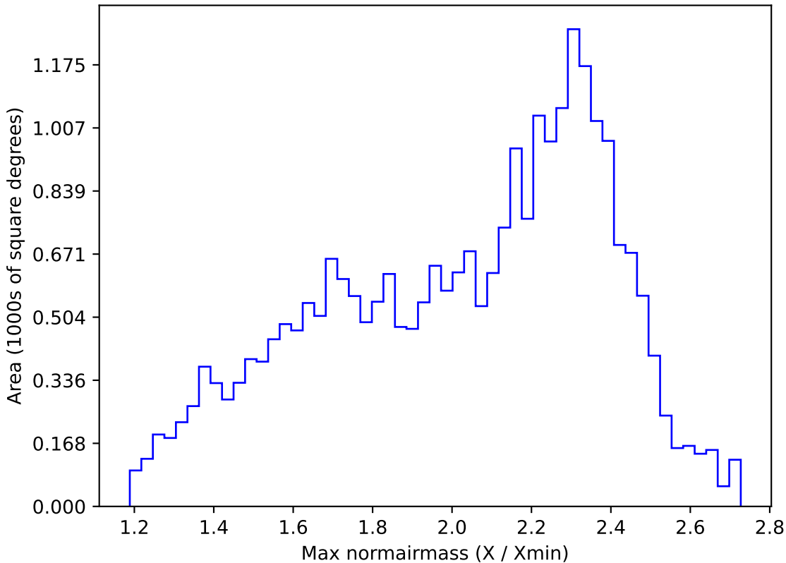
weather_cloudso18v3.4_10yrs All sky r band: Max normairmass
