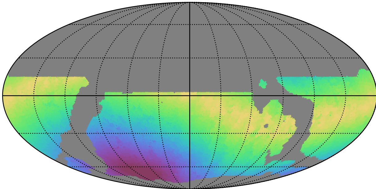
weather_cloudso18v3.4_10yrs WFD z band: Max moonDistance
