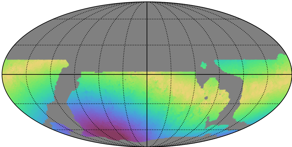
weather_cloudso18v3.4_10yrs WFD u band: Max moonDistance
