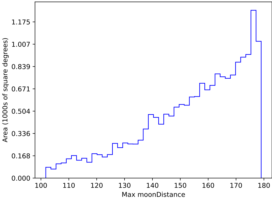
weather_cloudso18v3.4_10yrs WFD u band: Max moonDistance
