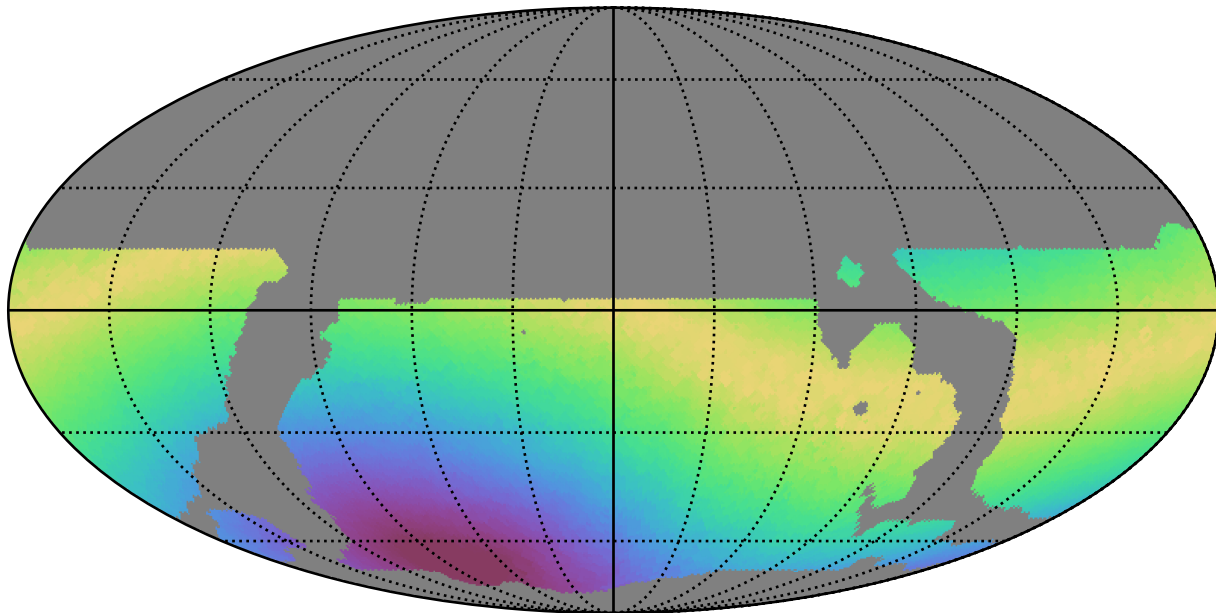
weather_cloudso18v3.4_10yrs WFD r band: Max moonDistance
