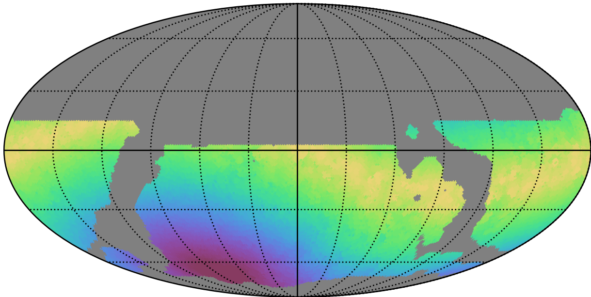
weather_cloudso18v3.4_10yrs WFD g band: Max moonDistance
