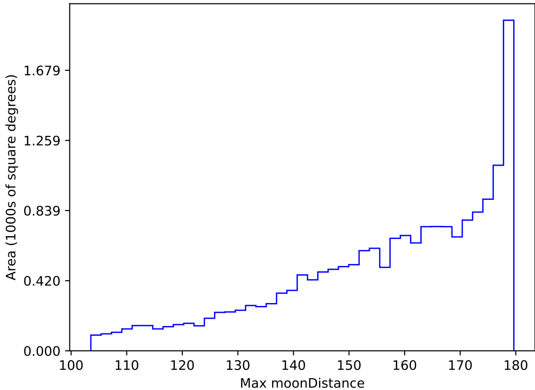
weather_cloudso18v3.4_10yrs WFD all bands: Max moonDistance
