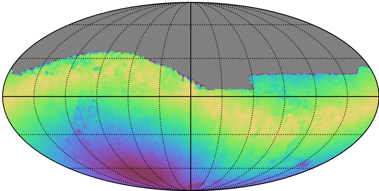
weather_cloudso18v3.4_10yrs All sky z band: Max moonDistance
