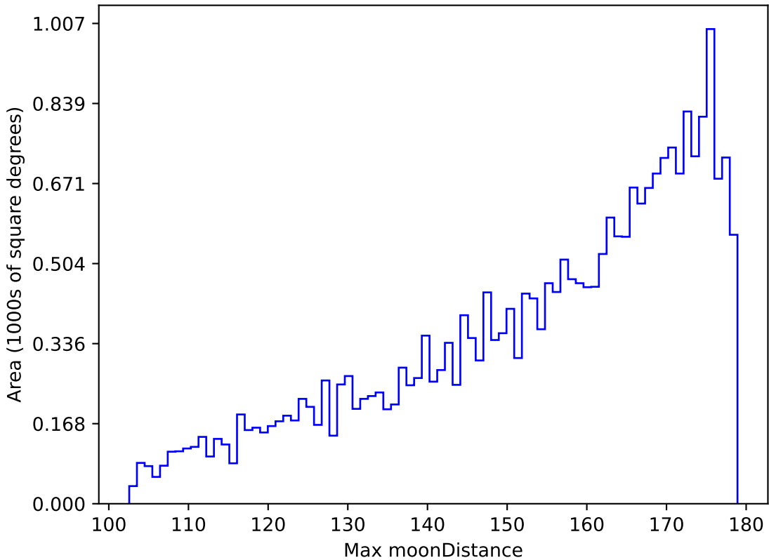
weather_cloudso18v3.4_10yrs All sky z band: Max moonDistance
