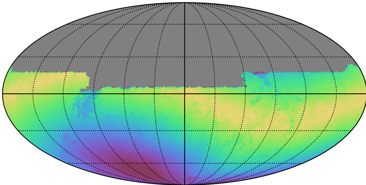
weather_cloudso18v3.4_10yrs All sky u band: Max moonDistance
