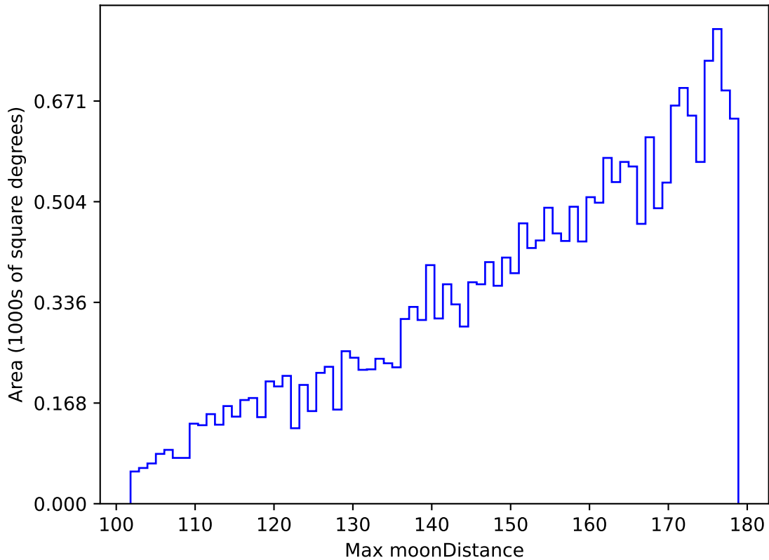
weather_cloudso18v3.4_10yrs All sky u band: Max moonDistance
