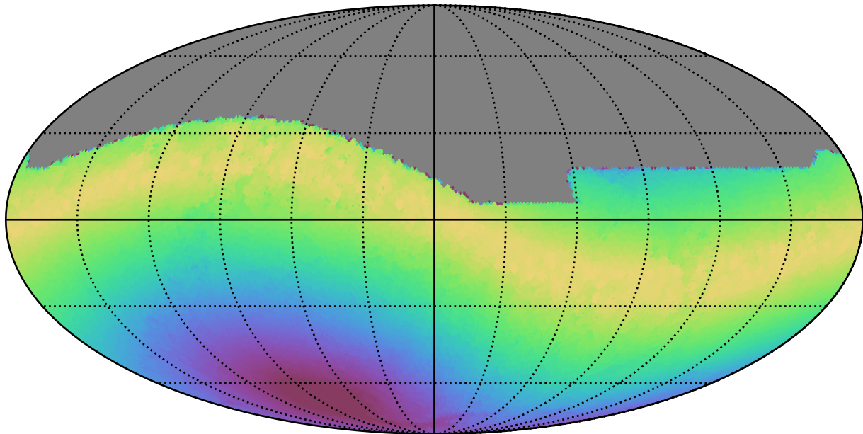
weather_cloudso18v3.4_10yrs All sky r band: Max moonDistance
