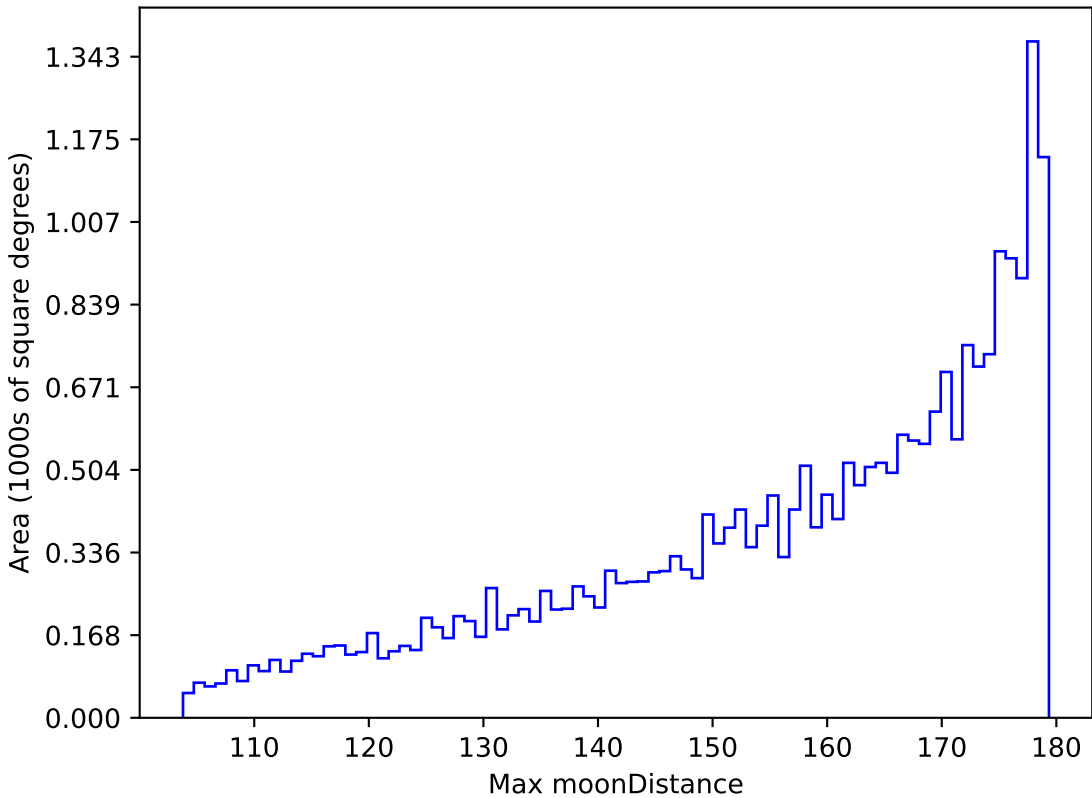
weather_cloudso18v3.4_10yrs All sky r band: Max moonDistance
