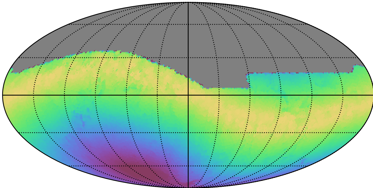
weather_cloudso18v3.4_10yrs All sky i band: Max moonDistance
