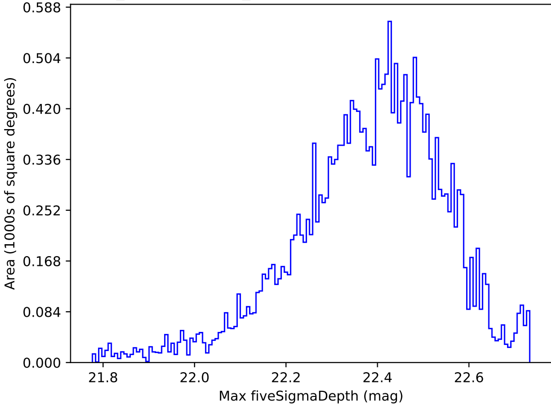
weather_cloudso18v3.4_10yrs Yr 1 y band: Max fiveSigmaDepth
