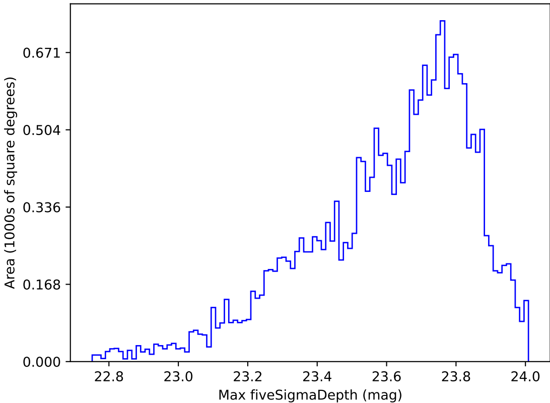
weather_cloudso18v3.4_10yrs Yr 1 u band: Max fiveSigmaDepth
