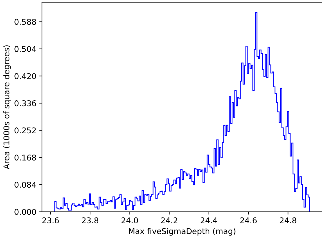
weather_cloudso18v3.4_10yrs Yr 1 r band: Max fiveSigmaDepth
