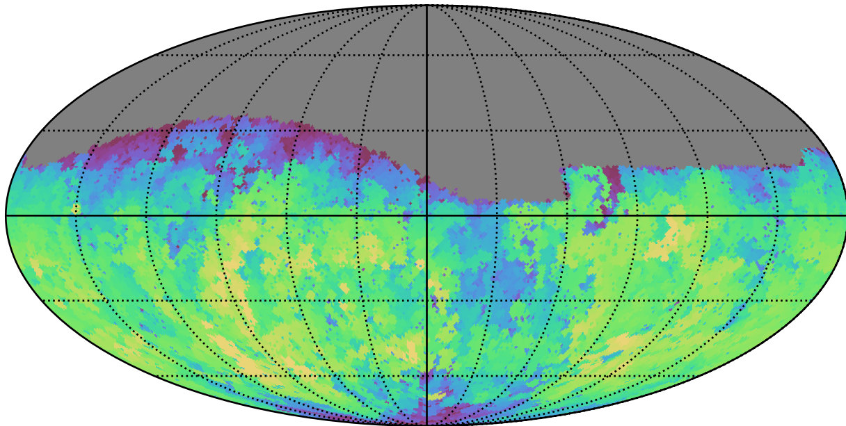
weather_cloudso18v3.4_10yrs Yr 1 g band: Max fiveSigmaDepth
