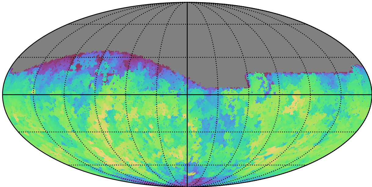
weather_cloudso18v3.4_10yrs Yr 1 all bands: Max fiveSigmaDepth
