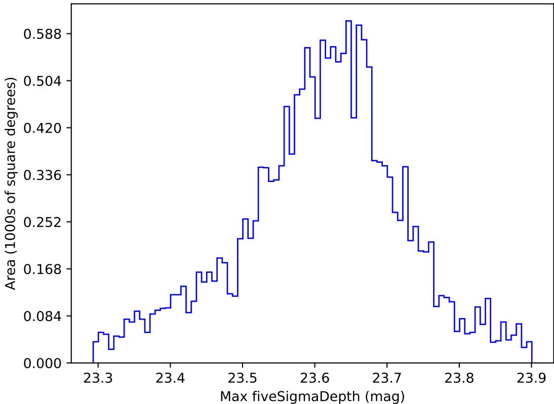
weather_cloudso18v3.4_10yrs WFD z band: Max fiveSigmaDepth
