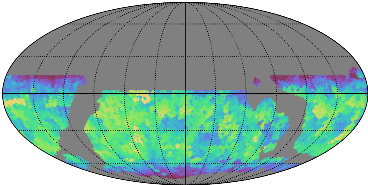
weather_cloudso18v3.4_10yrs WFD y band: Max fiveSigmaDepth
