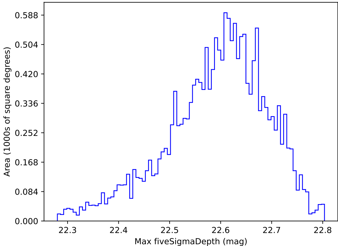
weather_cloudso18v3.4_10yrs WFD y band: Max fiveSigmaDepth
