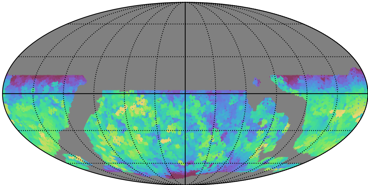
weather_cloudso18v3.4_10yrs WFD u band: Max fiveSigmaDepth
