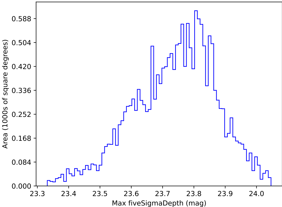
weather_cloudso18v3.4_10yrs WFD u band: Max fiveSigmaDepth
