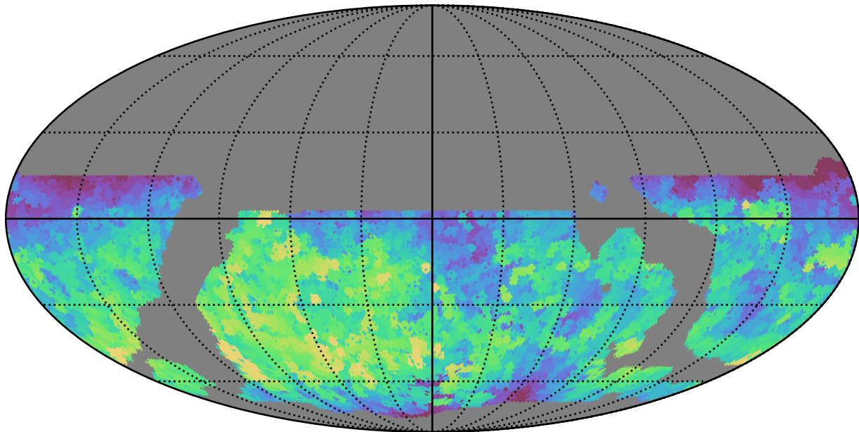
weather_cloudso18v3.4_10yrs WFD g band: Max fiveSigmaDepth
