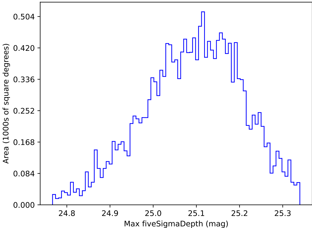
weather_cloudso18v3.4_10yrs WFD g band: Max fiveSigmaDepth
