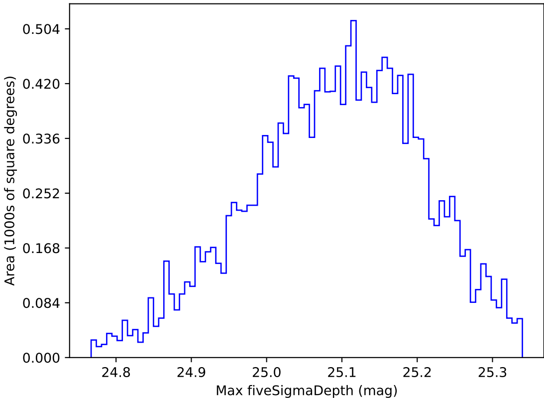
weather_cloudso18v3.4_10yrs WFD all bands: Max fiveSigmaDepth
