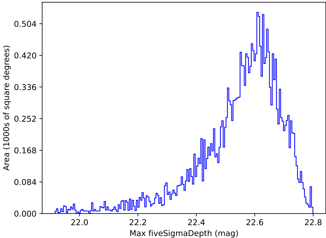
weather_cloudso18v3.4_10yrs All sky y band: Max fiveSigmaDepth
