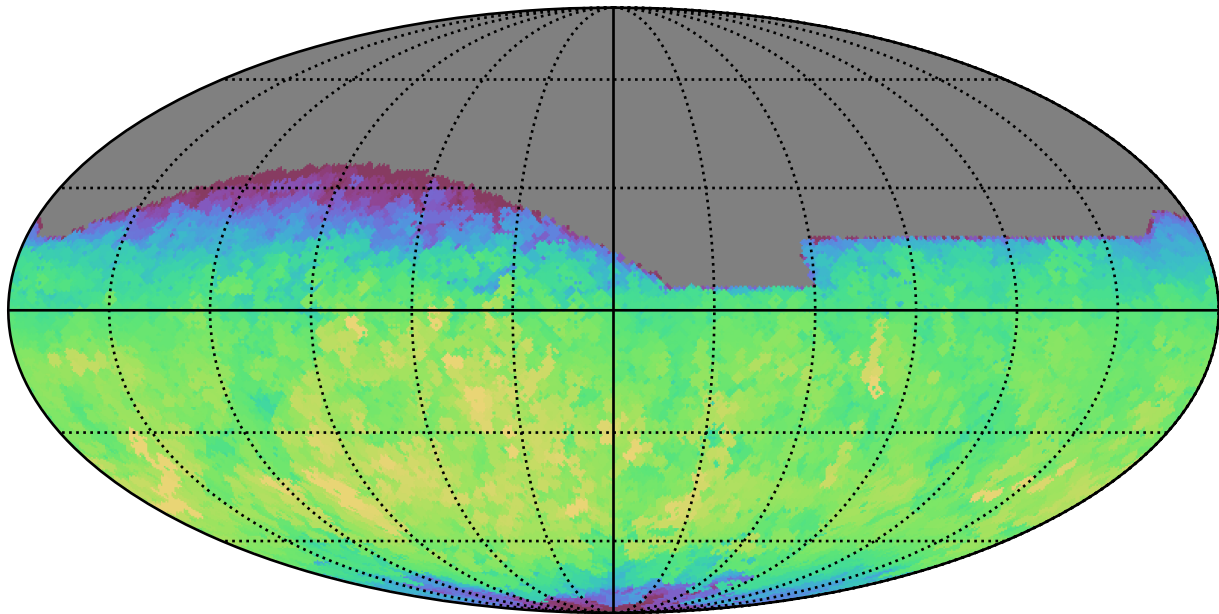
weather_cloudso18v3.4_10yrs All sky r band: Max fiveSigmaDepth
