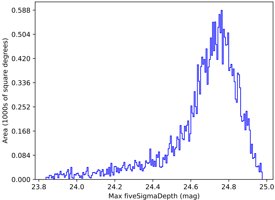
weather_cloudso18v3.4_10yrs All sky r band: Max fiveSigmaDepth
