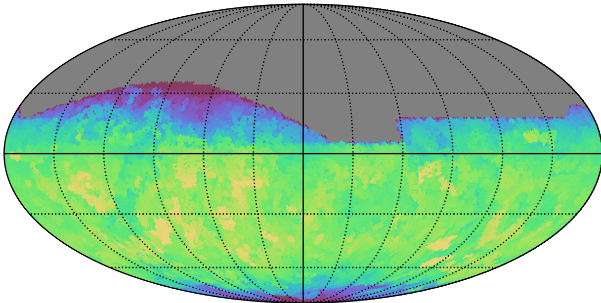
weather_cloudso18v3.4_10yrs All sky i band: Max fiveSigmaDepth
