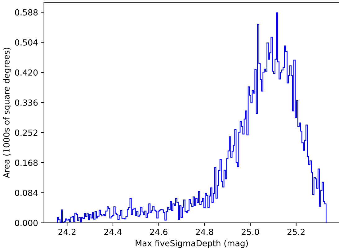
weather_cloudso18v3.4_10yrs All sky g band: Max fiveSigmaDepth
