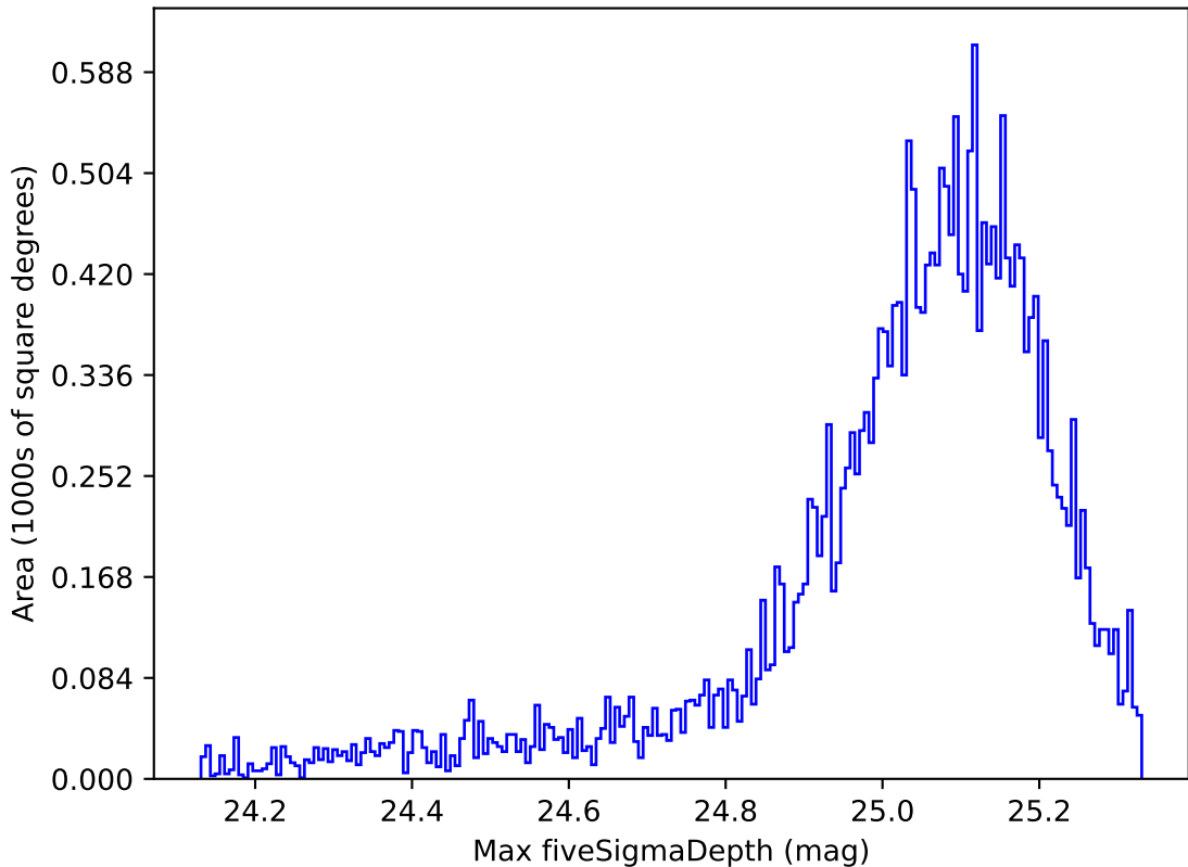
weather_cloudso18v3.4_10yrs All sky all bands: Max fiveSigmaDepth
