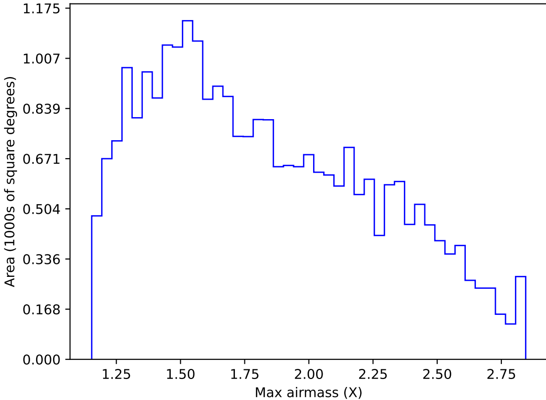
weather_cloudso18v3.4_10yrs Yr 1 z band: Max airmass
