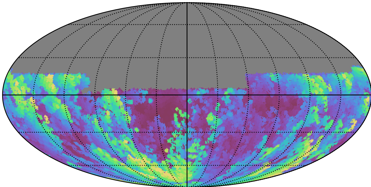
weather_cloudso18v3.4_10yrs Yr 1 y band: Max airmass
